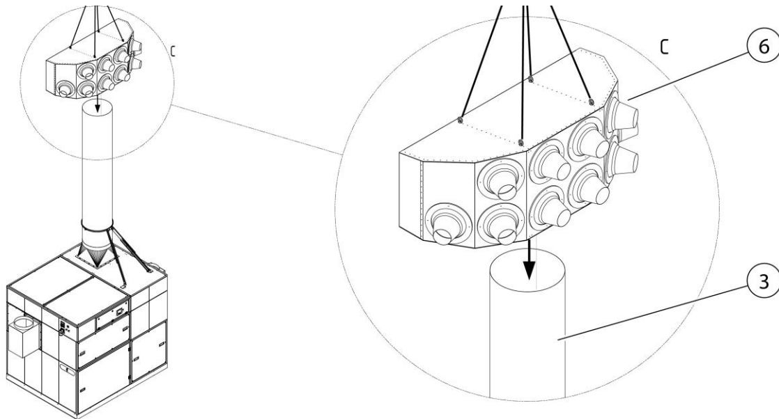
Fig. 13: Mounting – blower unit
