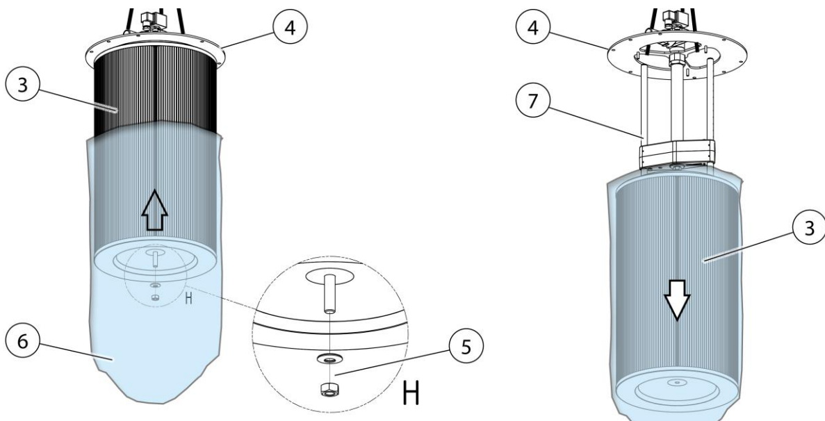
Fig. 46: Changing filters – removing the filter cartridge
