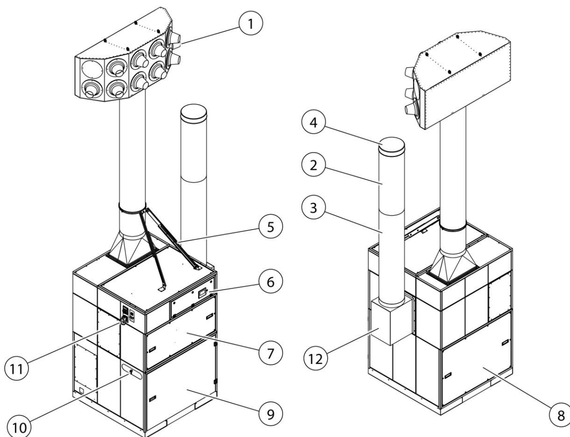
Fig. 4: Functional description - 998800461
