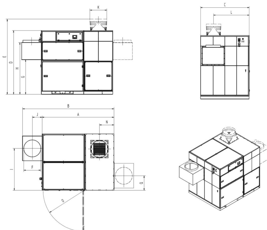
Fig. 56: Dimension sheets 998701370 (998800414, 998800463)
