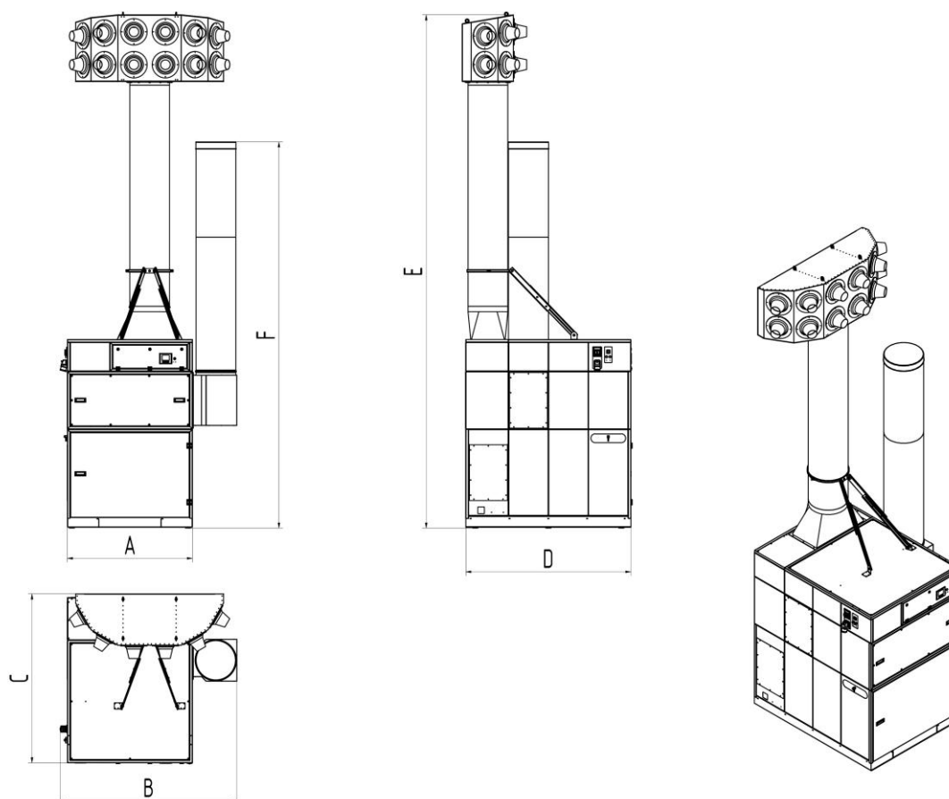
Fig. 61: Dimensions sheet – 998800462
