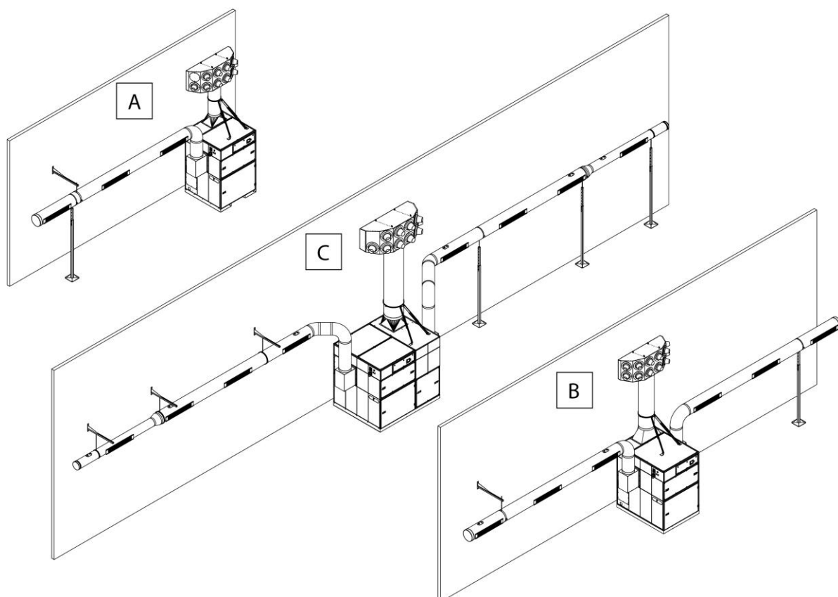
Fig. 11: Mounting – overview of product variants
