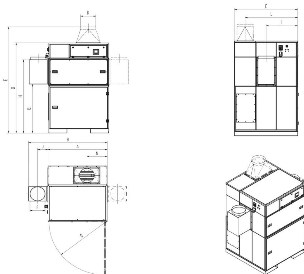
Fig. 54: Dimension sheets 998701372 (998800407, 998800461)
