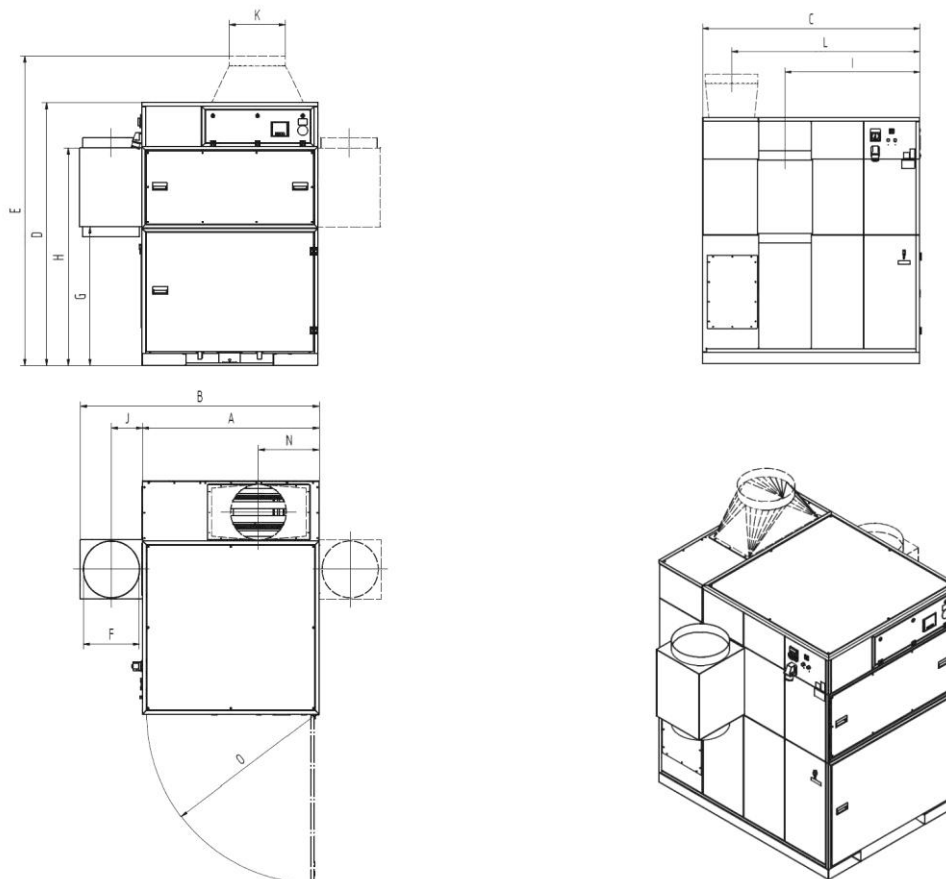
Fig. 55: Dimension sheets 998701371 (998800401, 998800462)
