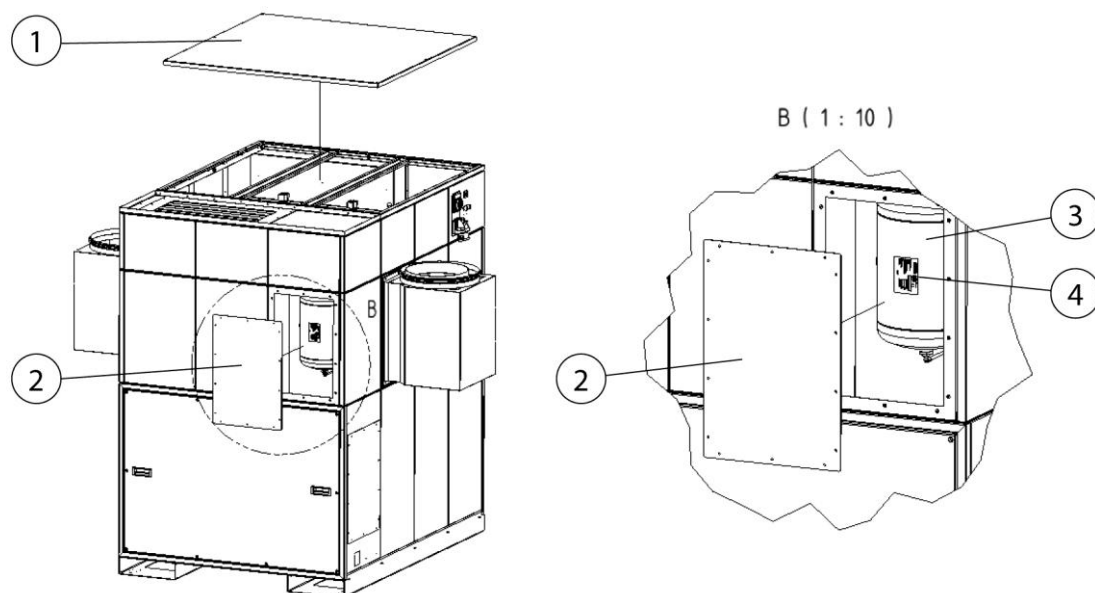
Fig. 52: Access to compressed air vessel
